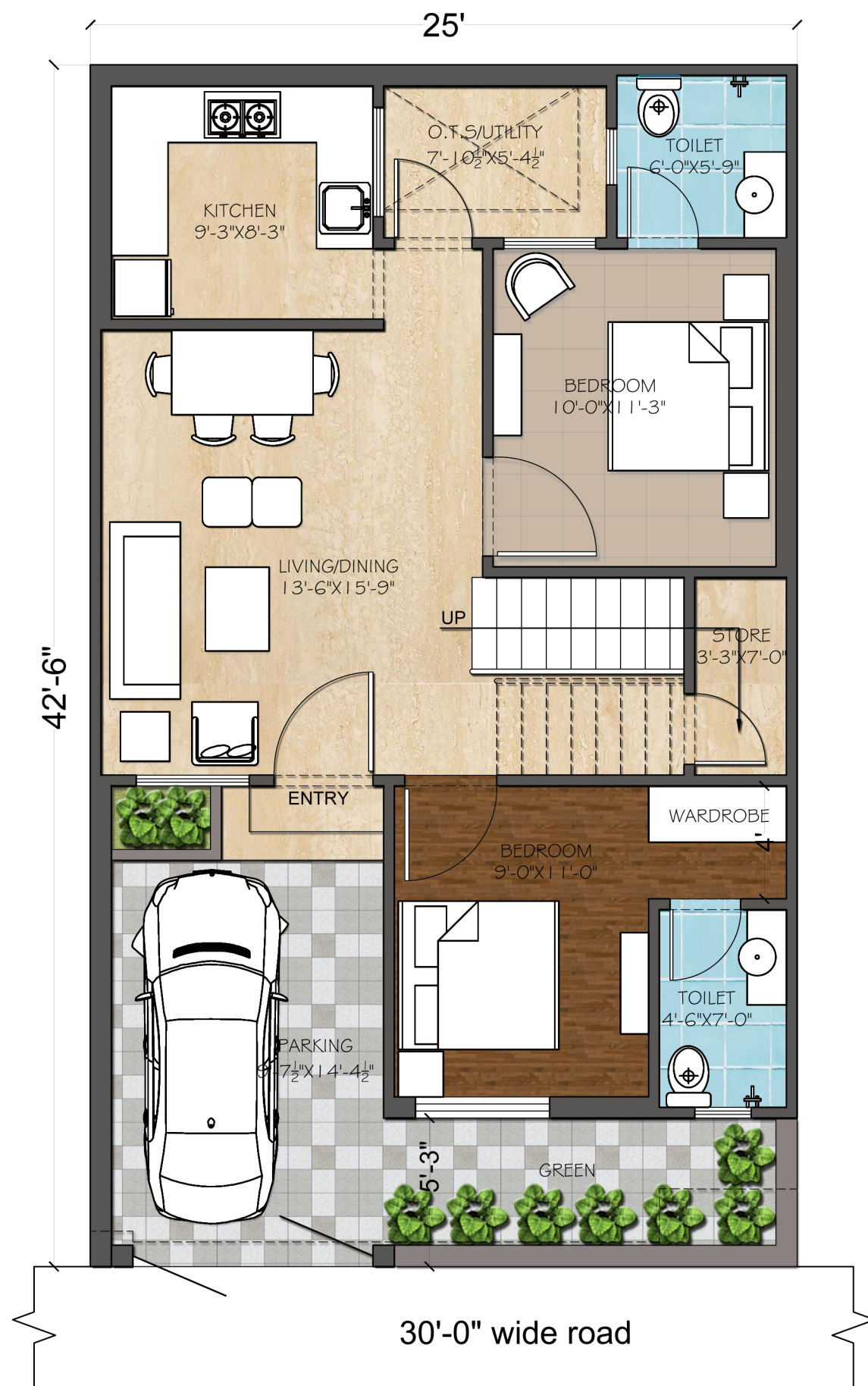
GROUND FLOOR COVERED AREA: 1000.15 SQ.FT.
